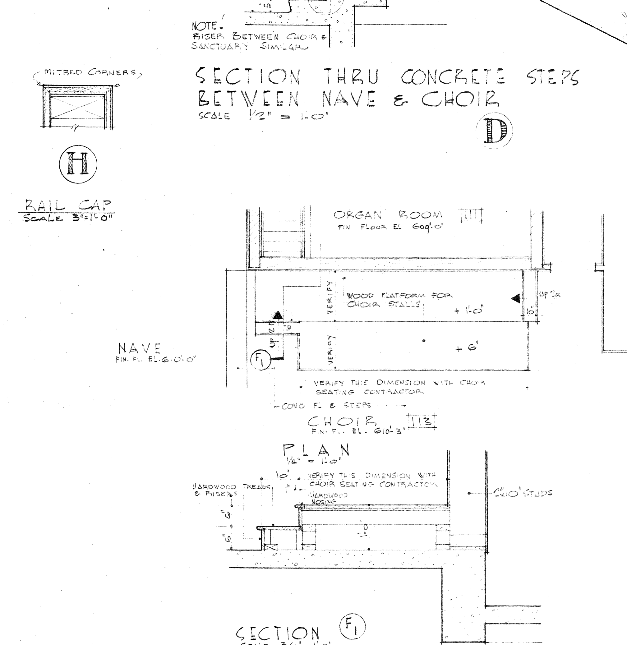
DETAILS OF WOOD PLATFORM FOR CHOIR STALLS
