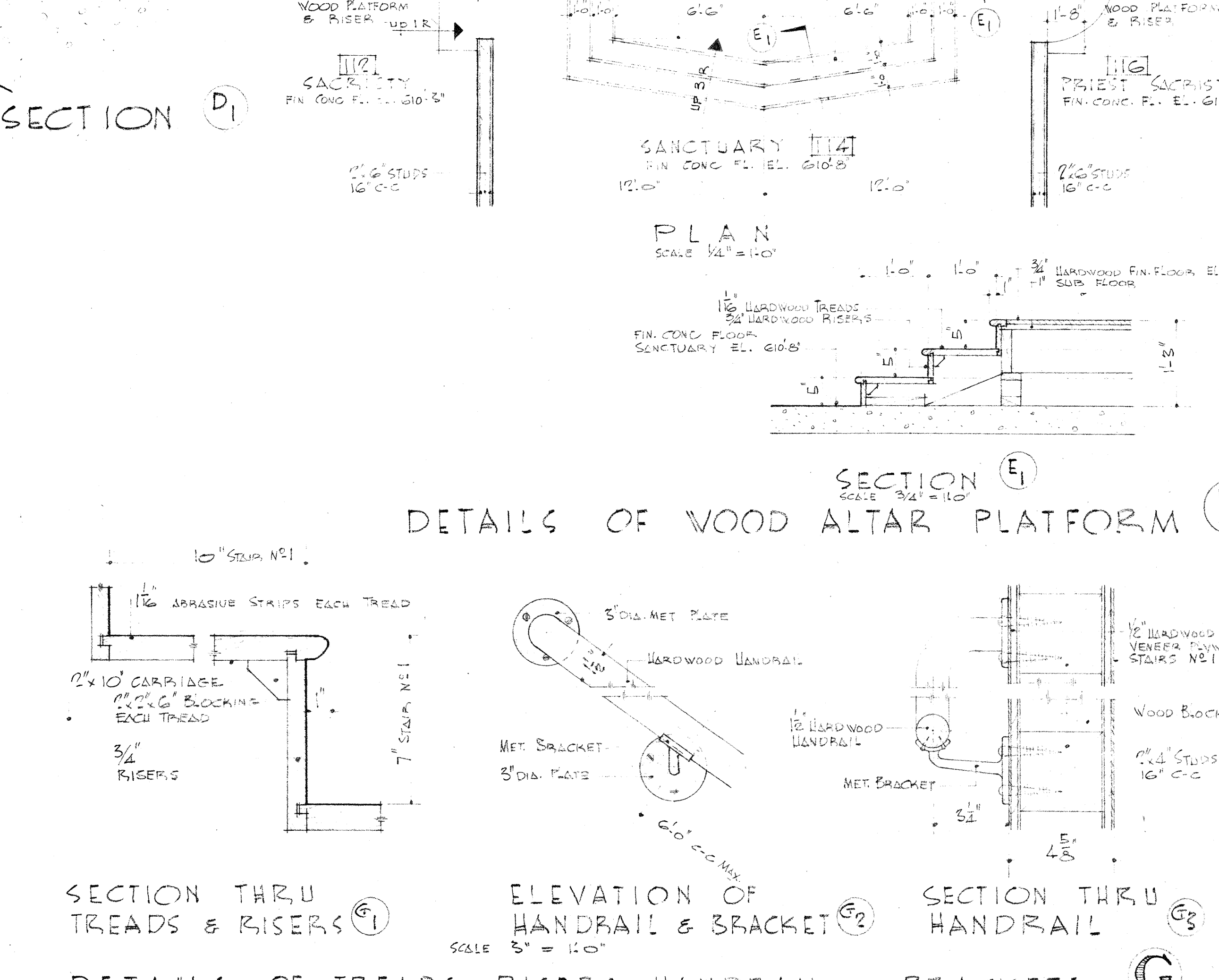
DETAILS OF TREADS-RISERS HANDRAIL & BRACKETS
